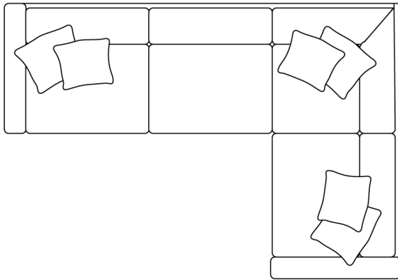
LARGE CORNER SOFA H950 W2440 D1720
