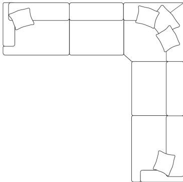
LARGE CORNER SOFA H980 W2750 D2750
