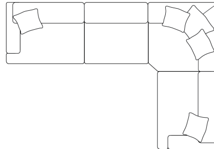
SMALL CORNER SOFA H980 W2750 D2060
